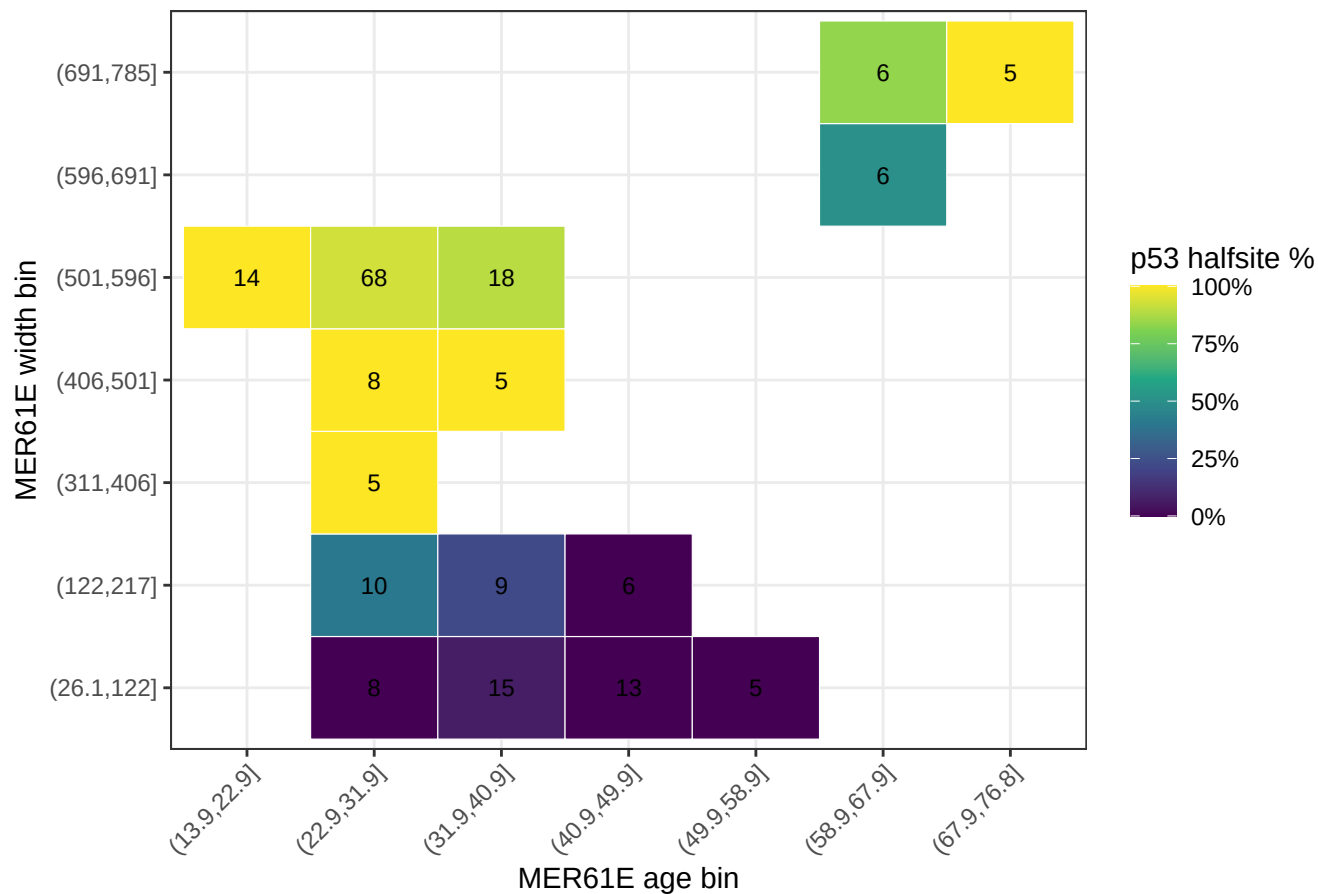
p53 halfsite enrichment across MER61E age and width
