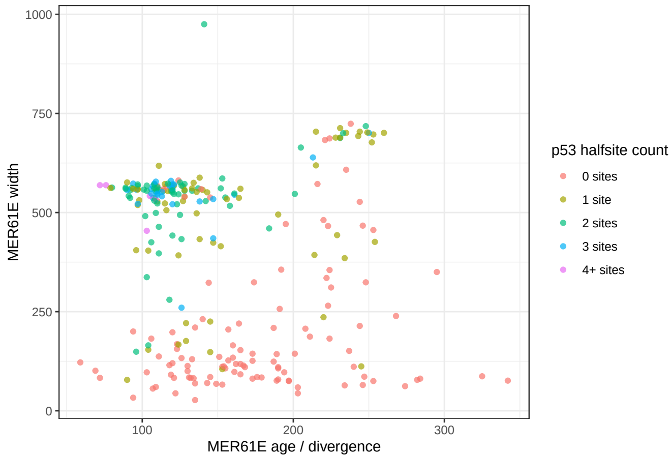
MER61E width and age by p53 halvesite count
