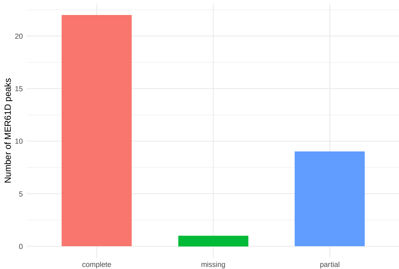
ChromHMM state coverage completeness for MER61D
