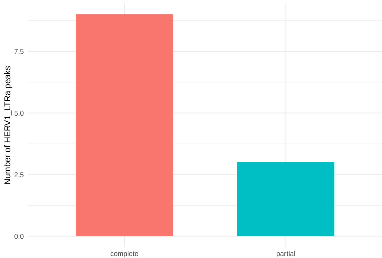
ChromHMM state coverage completeness for HERV1_LTRa
