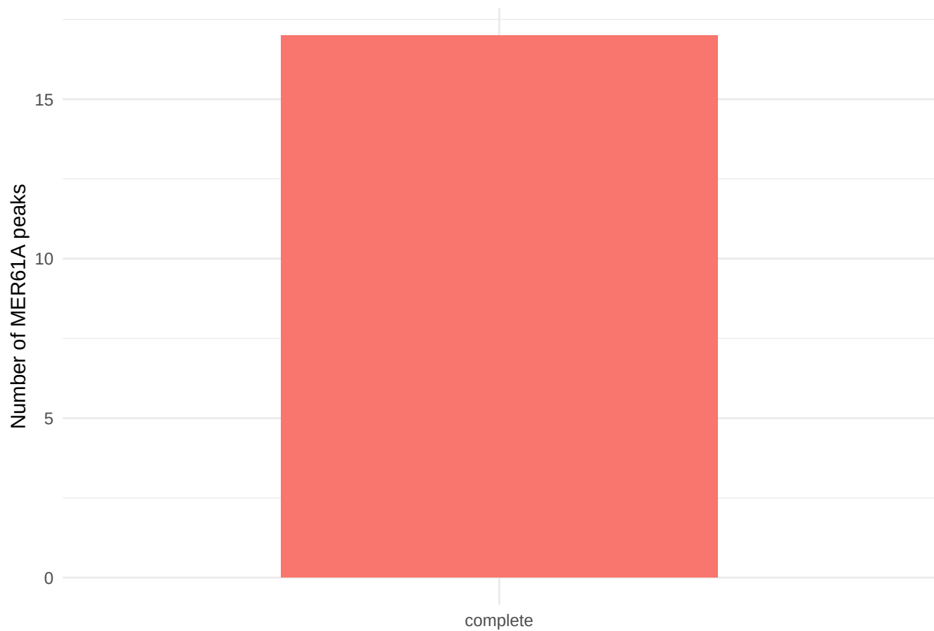
ChromHMM state coverage completeness for MER61A
