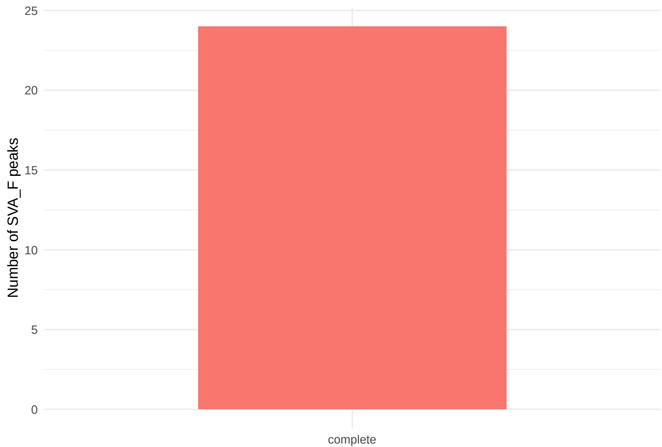
ChromHMM state coverage completeness for SVA_F
