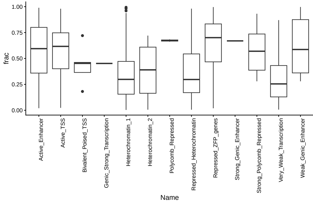
Fraction of MER61E elements assigned to each ChromHMM state (all exactly two-state overlaps)
