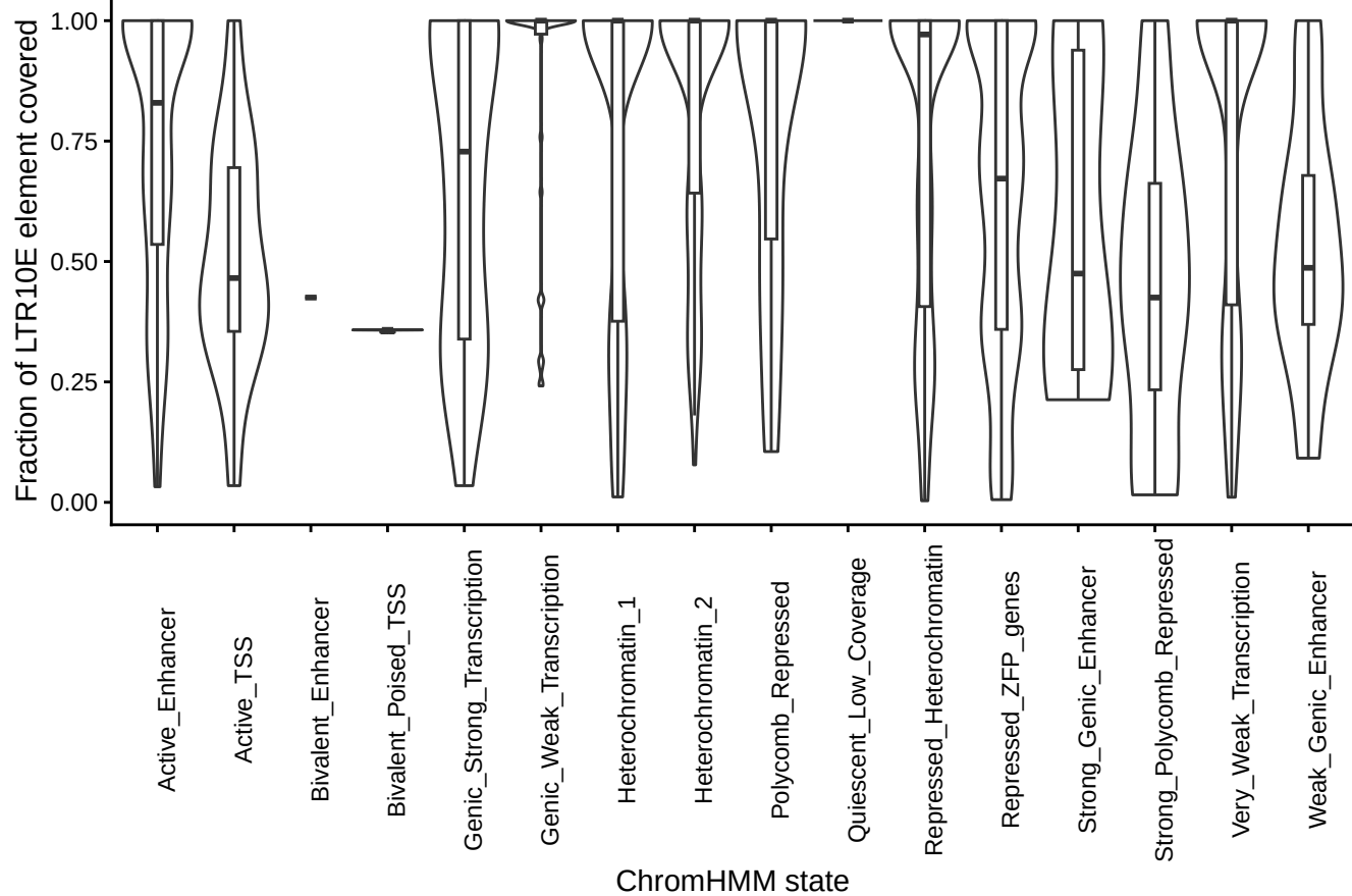
Distribution of nonzero ChromHMM state fractions across all LTR10E elements
