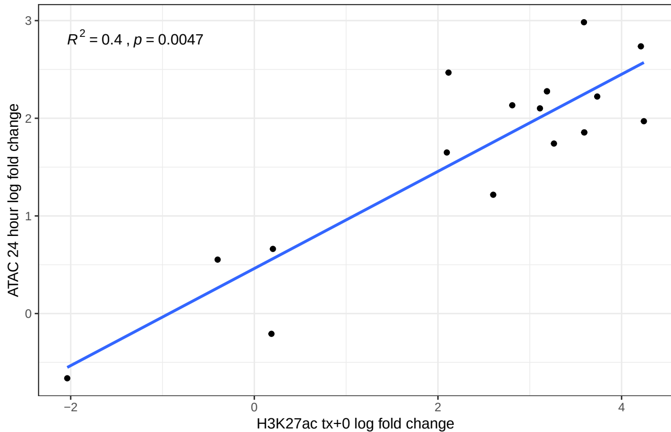
Scatterplot with Spearmann correlation of regions overlapping the same LTR10Es
