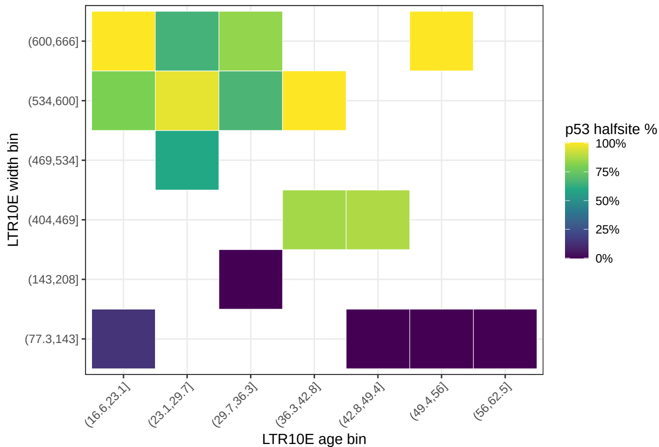
p53 halfsite enrichment across LTR10E age and width
