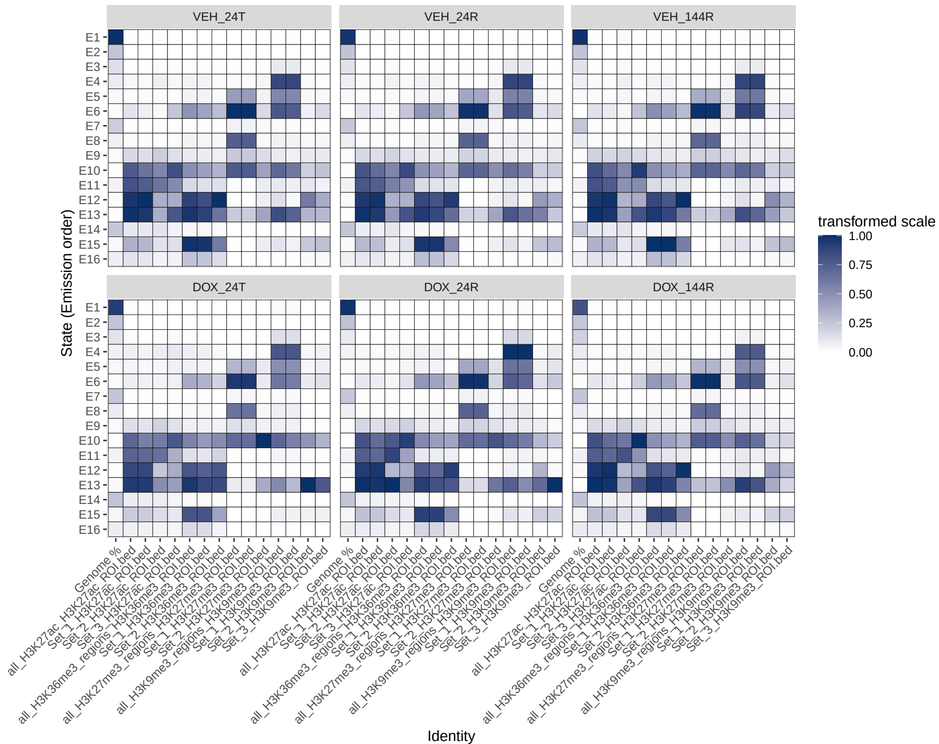
Cormotif across states
