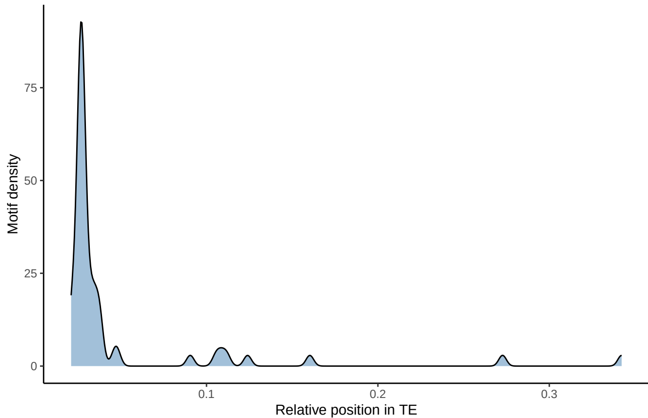
Motif distribution: fimo_out_24 MEME-20
