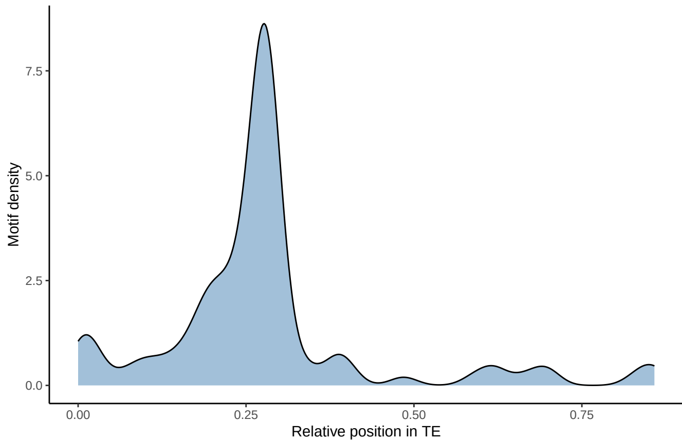
Motif distribution: fimo_out_33 MEME-21
