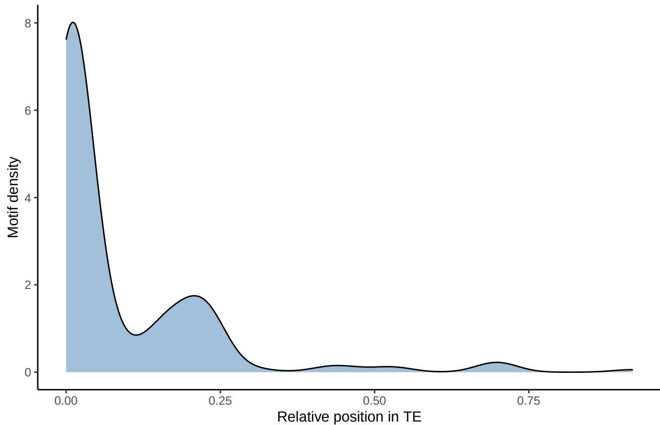
Motif distribution: fimo_out_14 STREME-5
