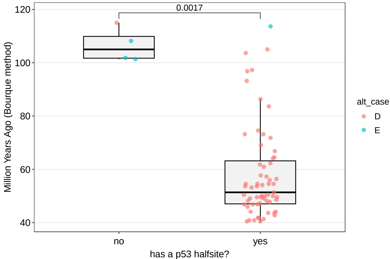
MER61E MYA (Bourque method) of integrants overlapping my H3K27ac data and looking at p53 halvesites
