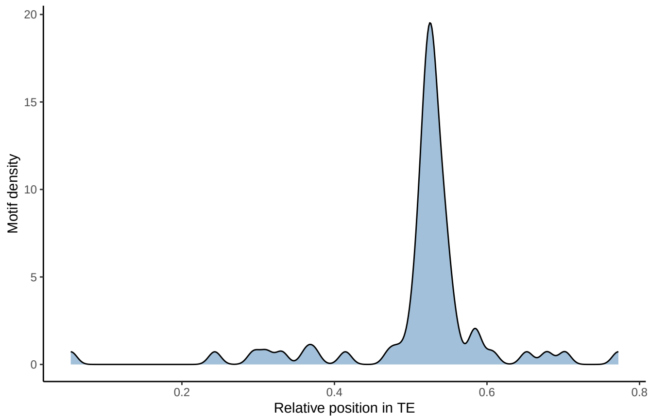
Motif distribution: fimo_out_22 MEME-18
