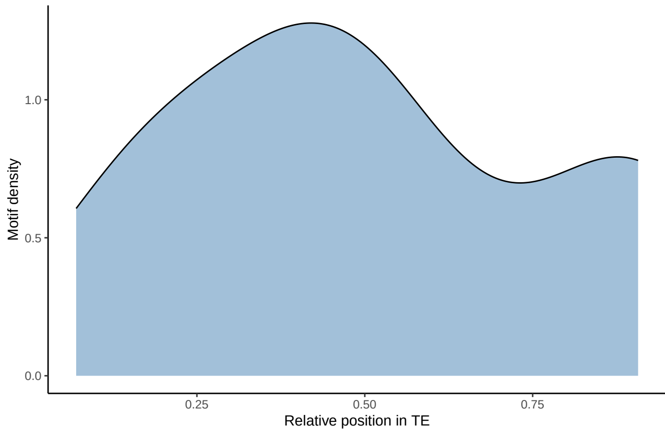
Motif distribution: fimo_out_51 MEME-44
