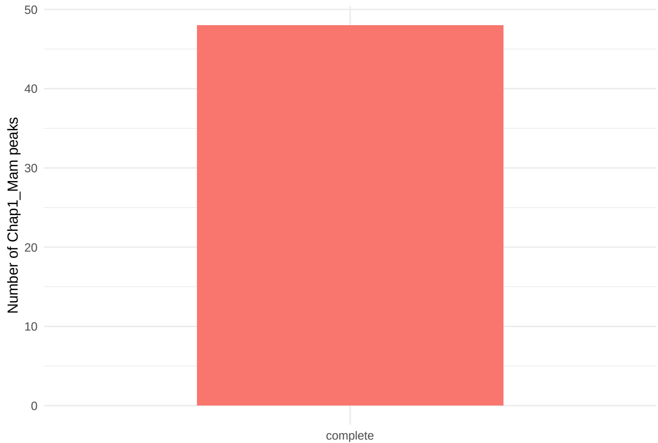
ChromHMM state coverage completeness for Chap1_Mam
