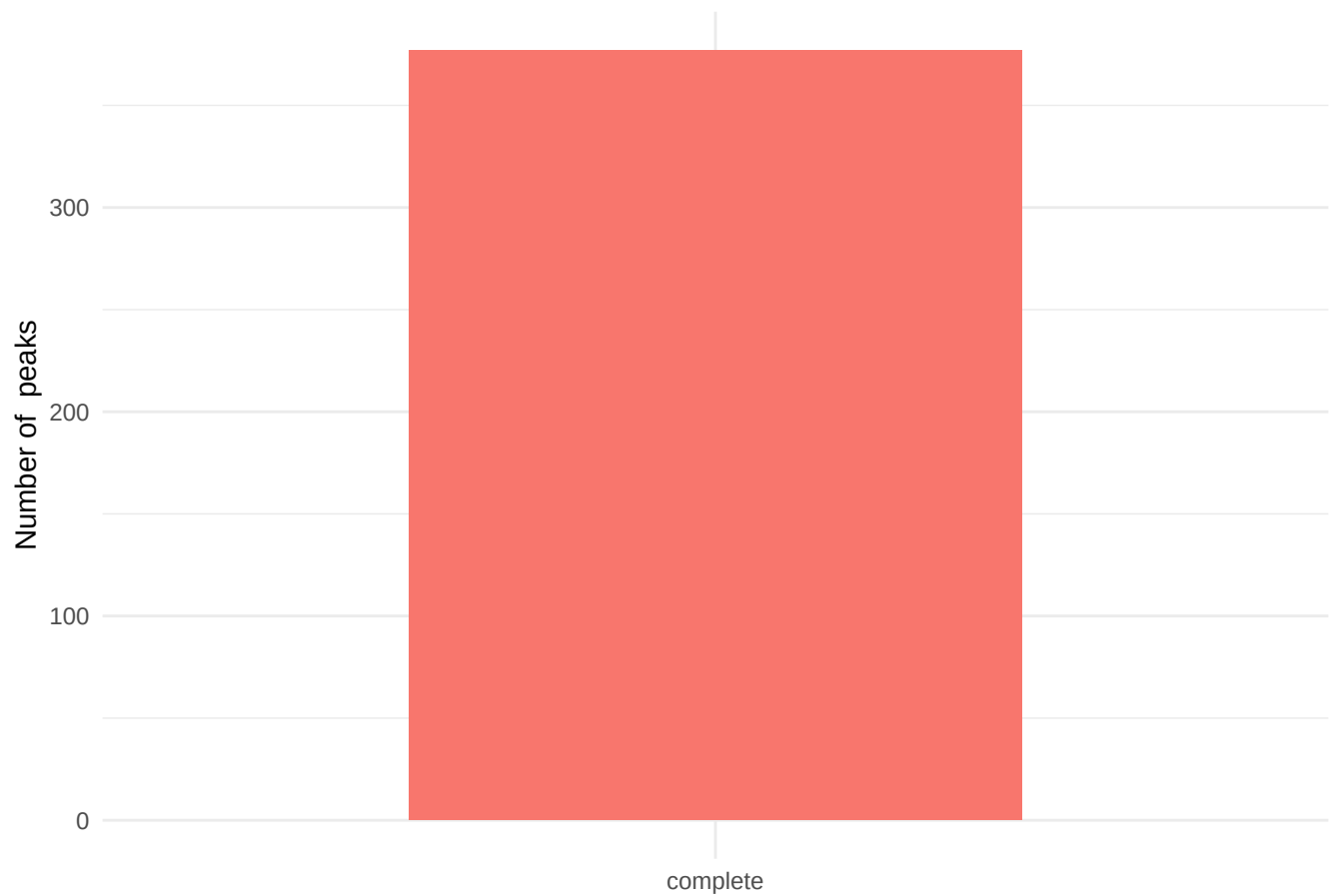
ChromHMM state coverage completeness for KZFP TSS \pm 50bp
