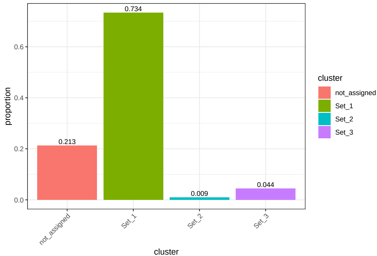
Proportion of ROIs by cluster
