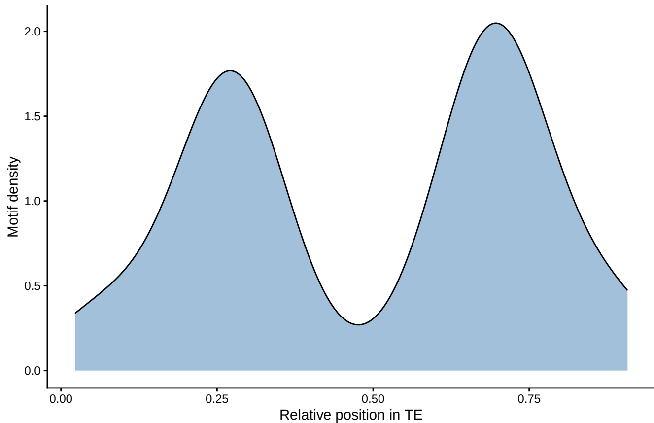
TP53 halfsite motif distribution: MER61C_ERV1_LTR_fimo NA
