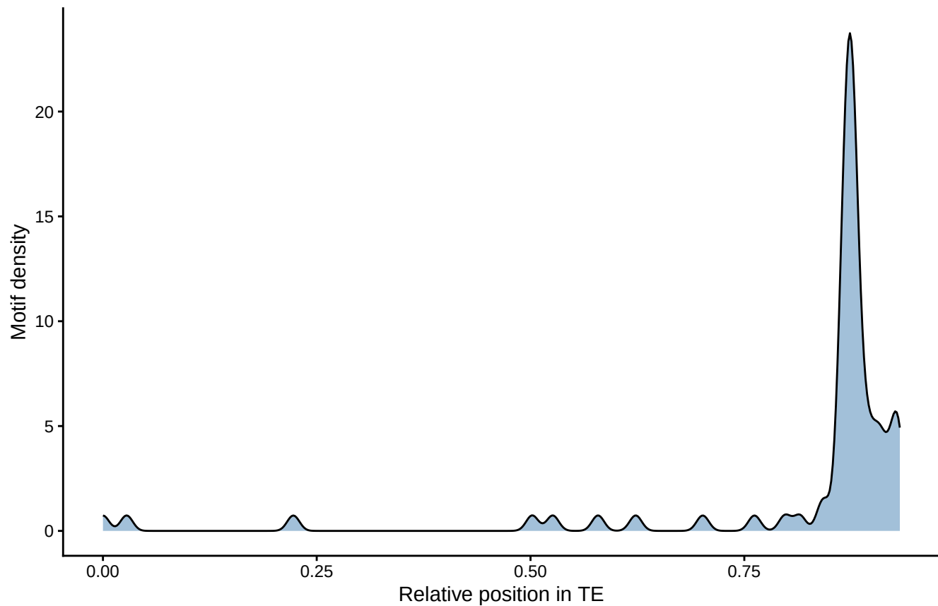
Motif distribution: fimo_out_25 MEME-9
