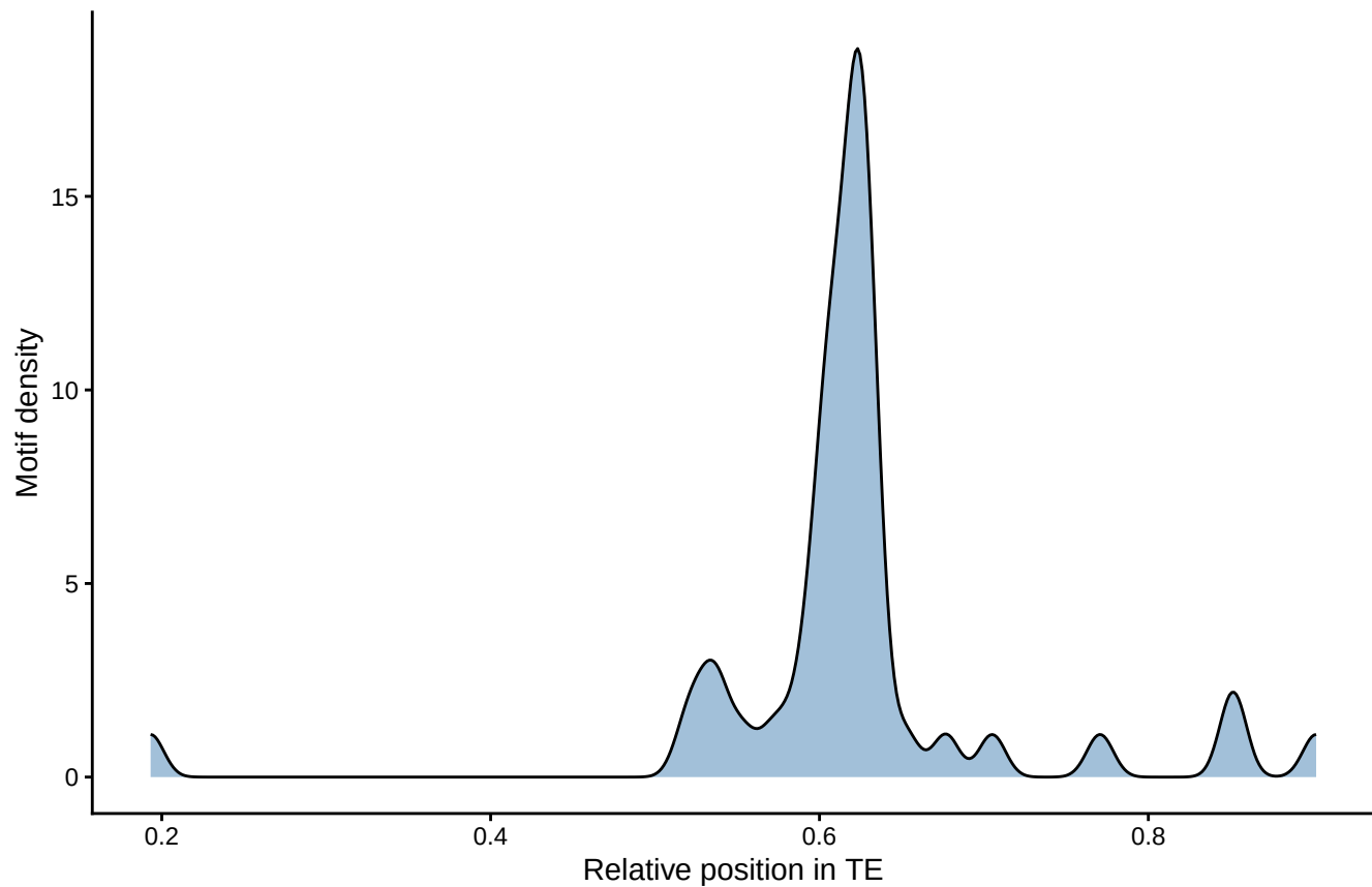
Motif distribution: fimo_out_47 MEME-36
