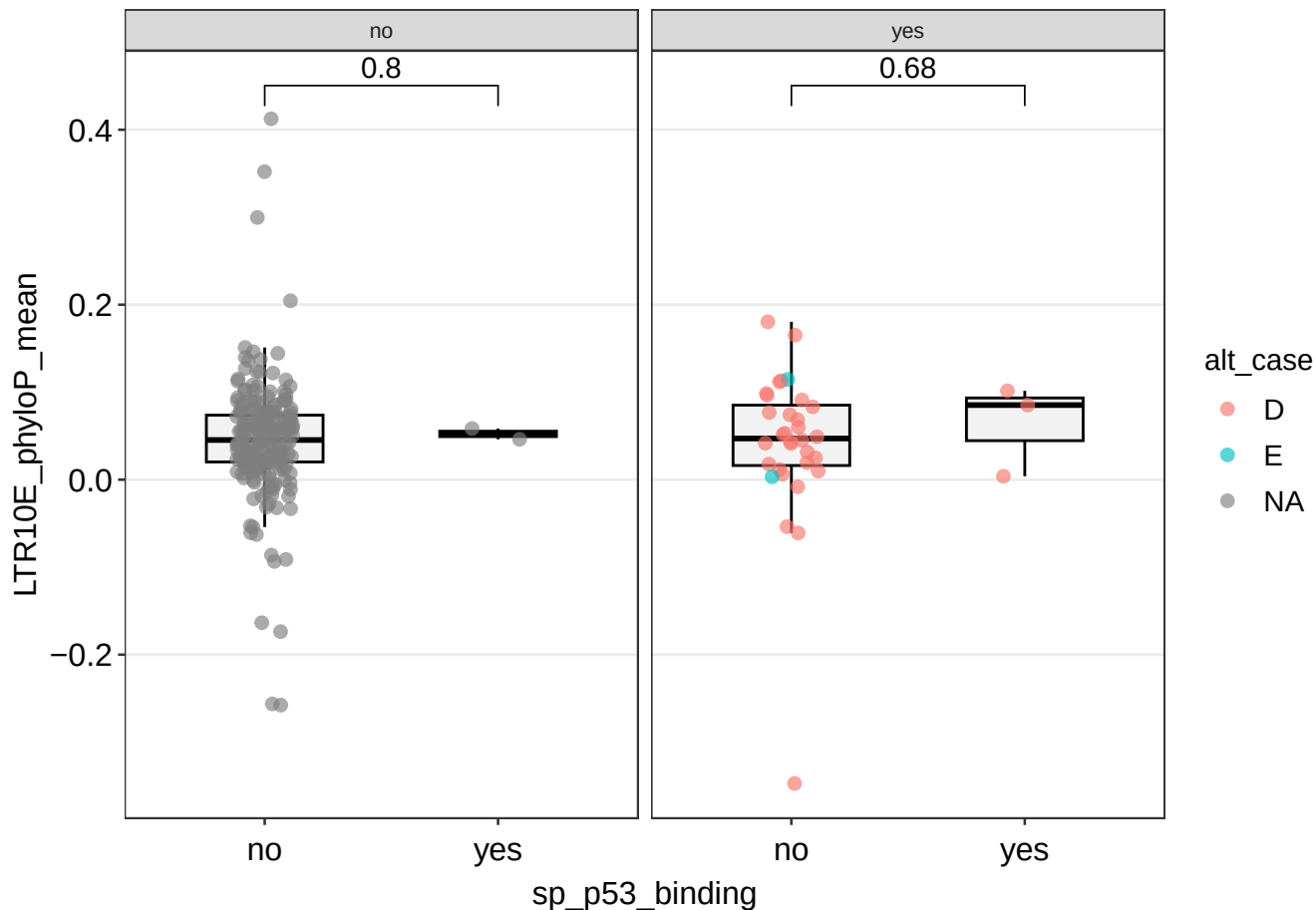
mean LTR10E phyloP which overlap p53 ChIP data
