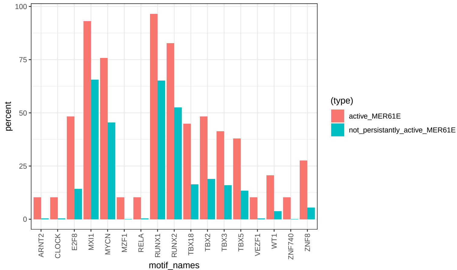
expressed TF enrichment in persistantly activated TEs
