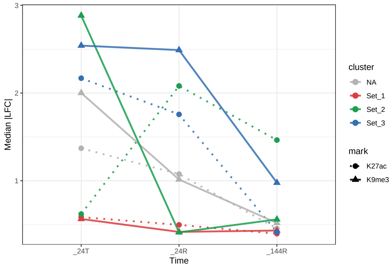
Both histones, absolute LFC overlapping LTR:ERVL
