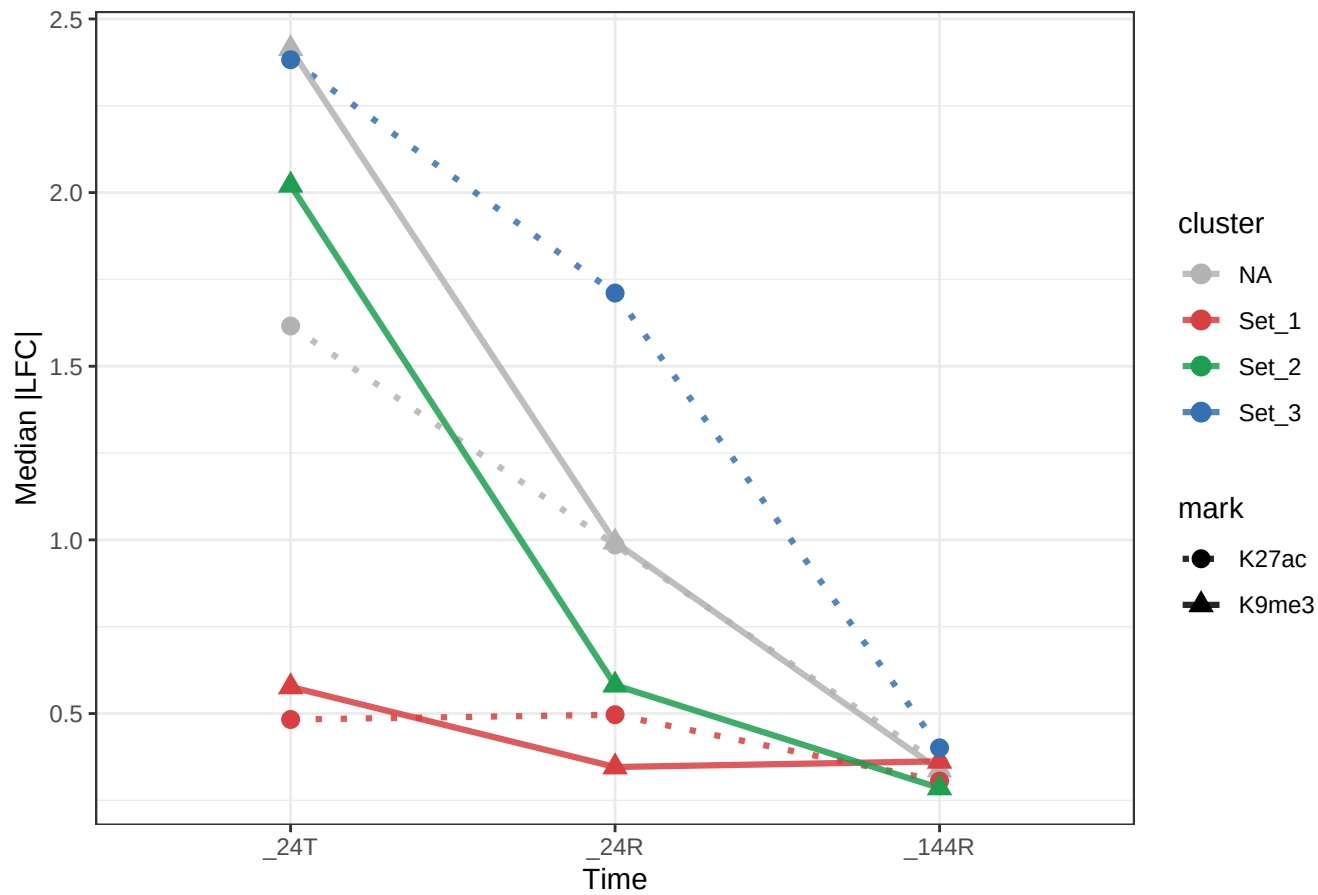
Both histones, absolute LFC overlapping LTR:ERVK
