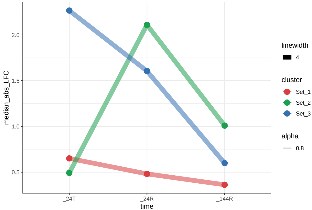
K27ac absolute LFC overlapping LTR:Gypsy
