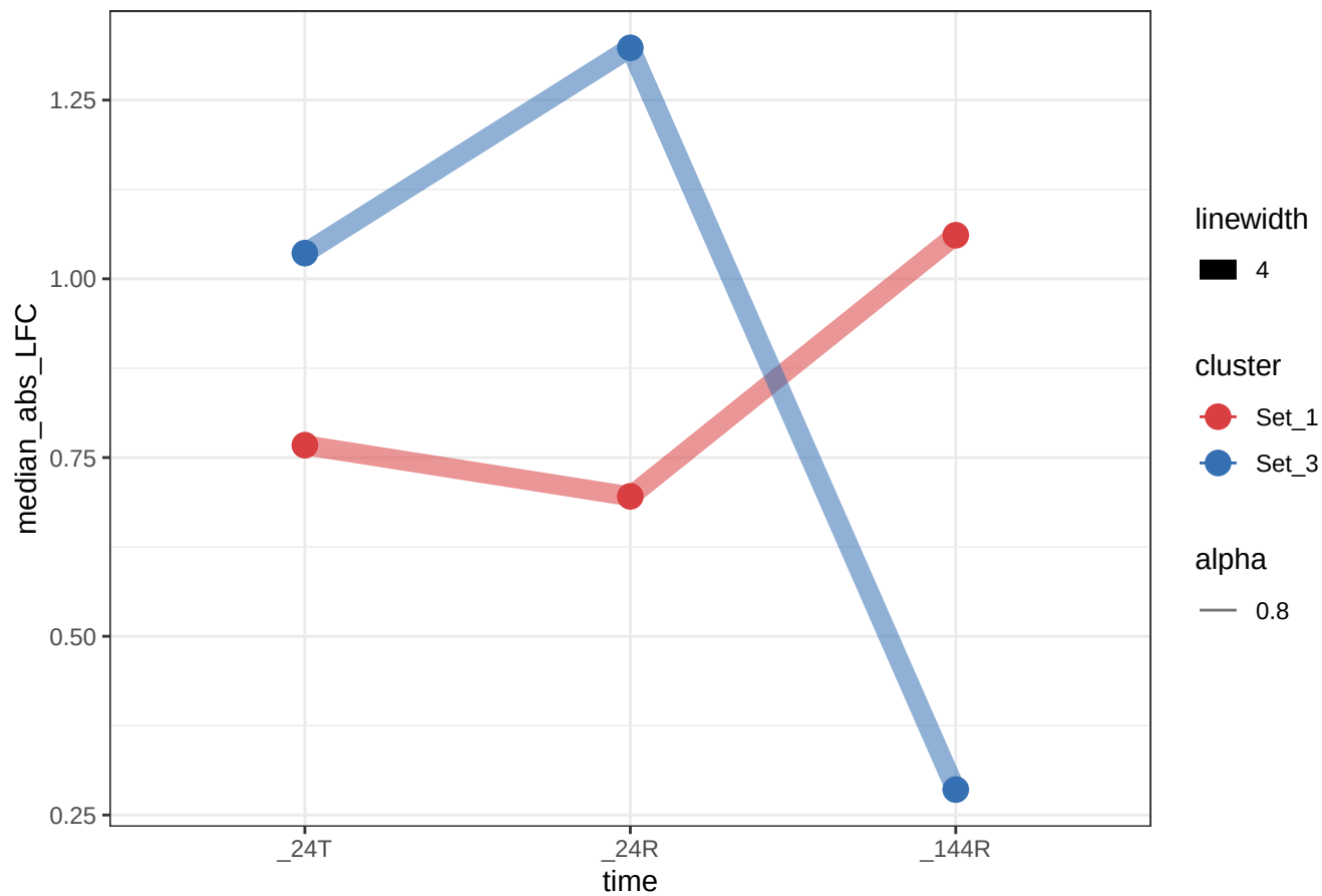
K27ac absolute LFC overlapping LTR:LTR
