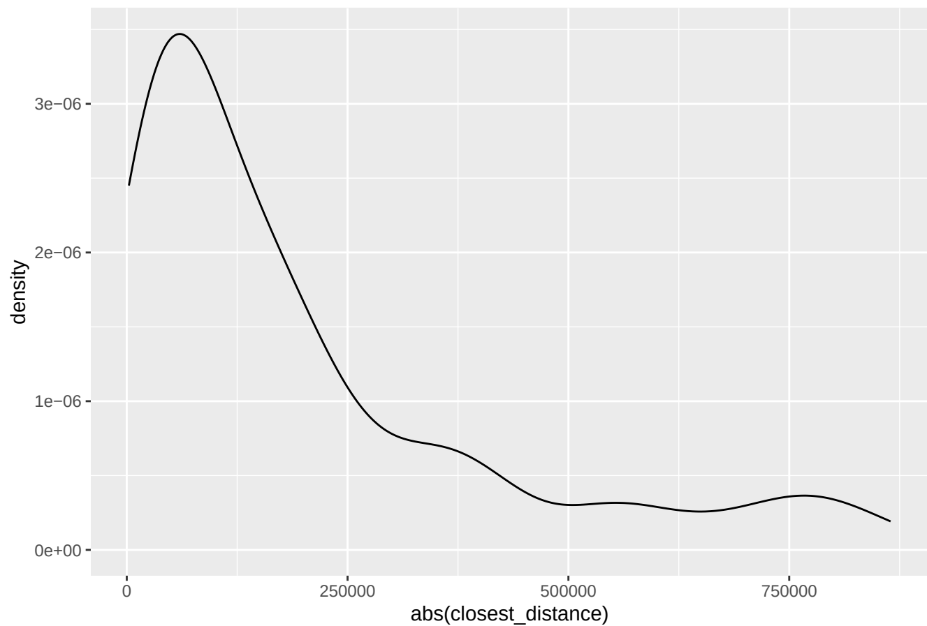
density of MER61E TEs distance to expressed gene (GREAT)
