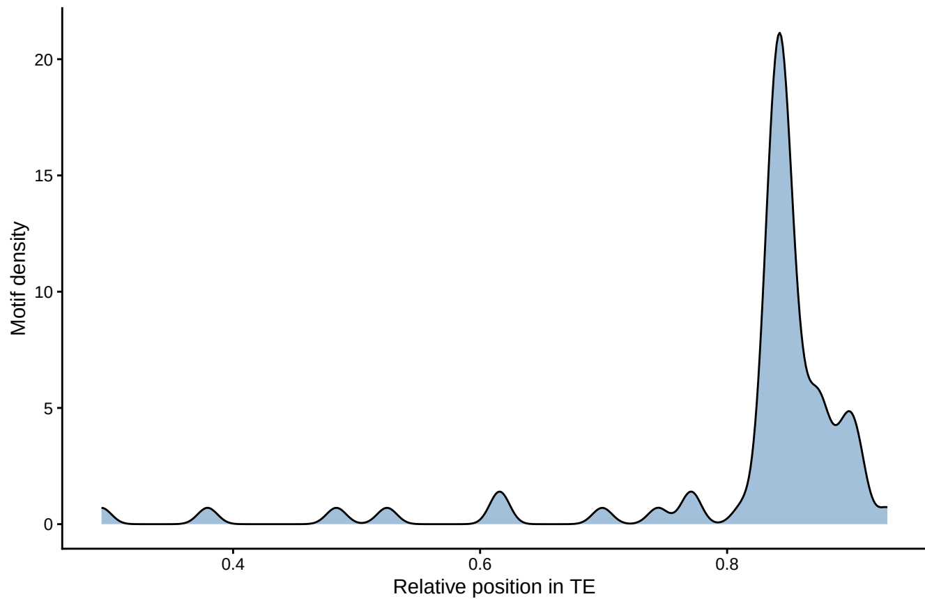
Motif distribution: fimo_out_18 MEME-17
