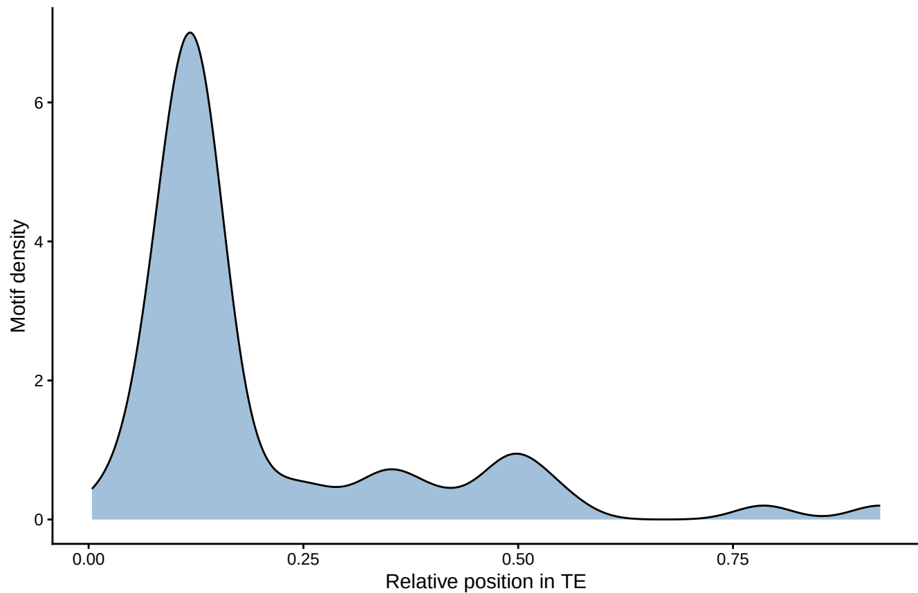
Motif distribution: fimo_out_40 STREME-33
