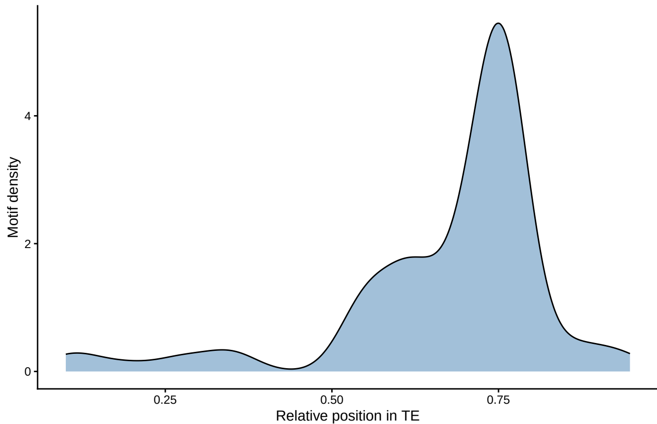
Motif distribution: fimo_out_6 STREME-13
