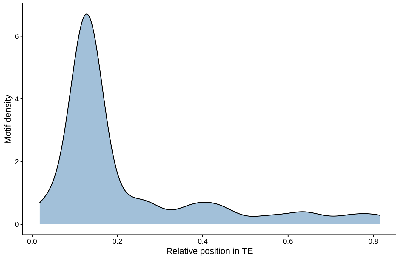
Motif distribution: fimo_out_9 STREME-2
