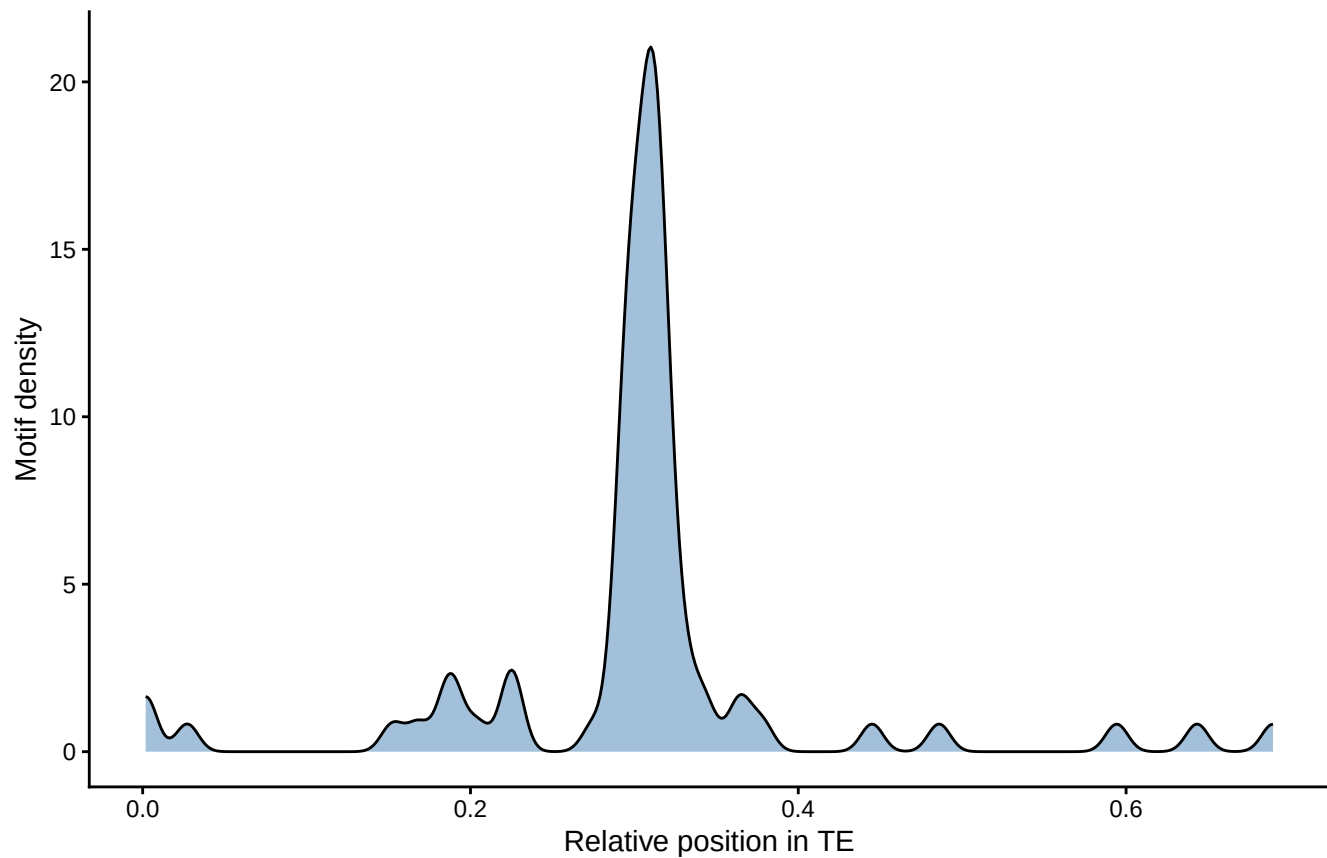
Motif distribution: fimo_out_16 STREME-29
