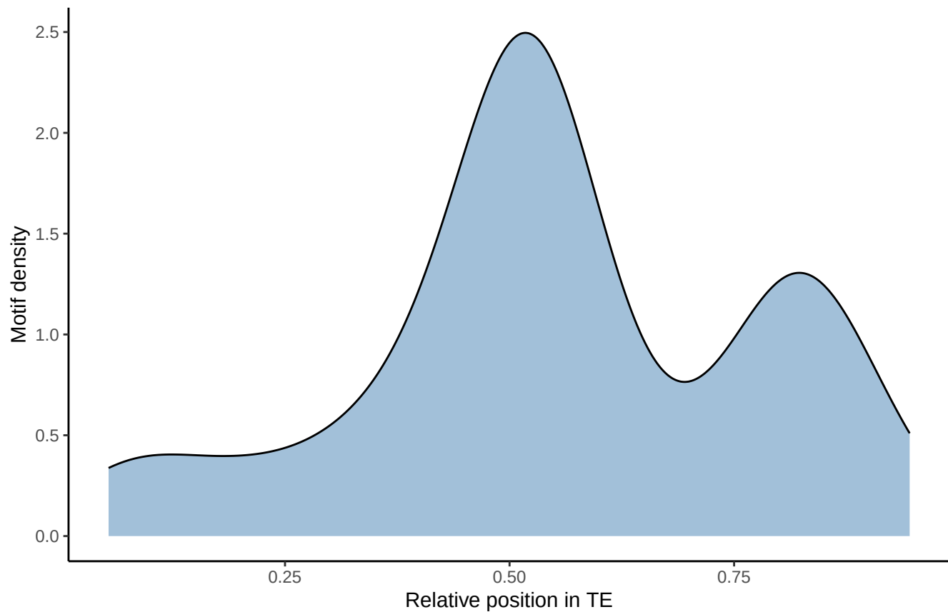
Motif distribution: fimo_out_1 MEME-4
