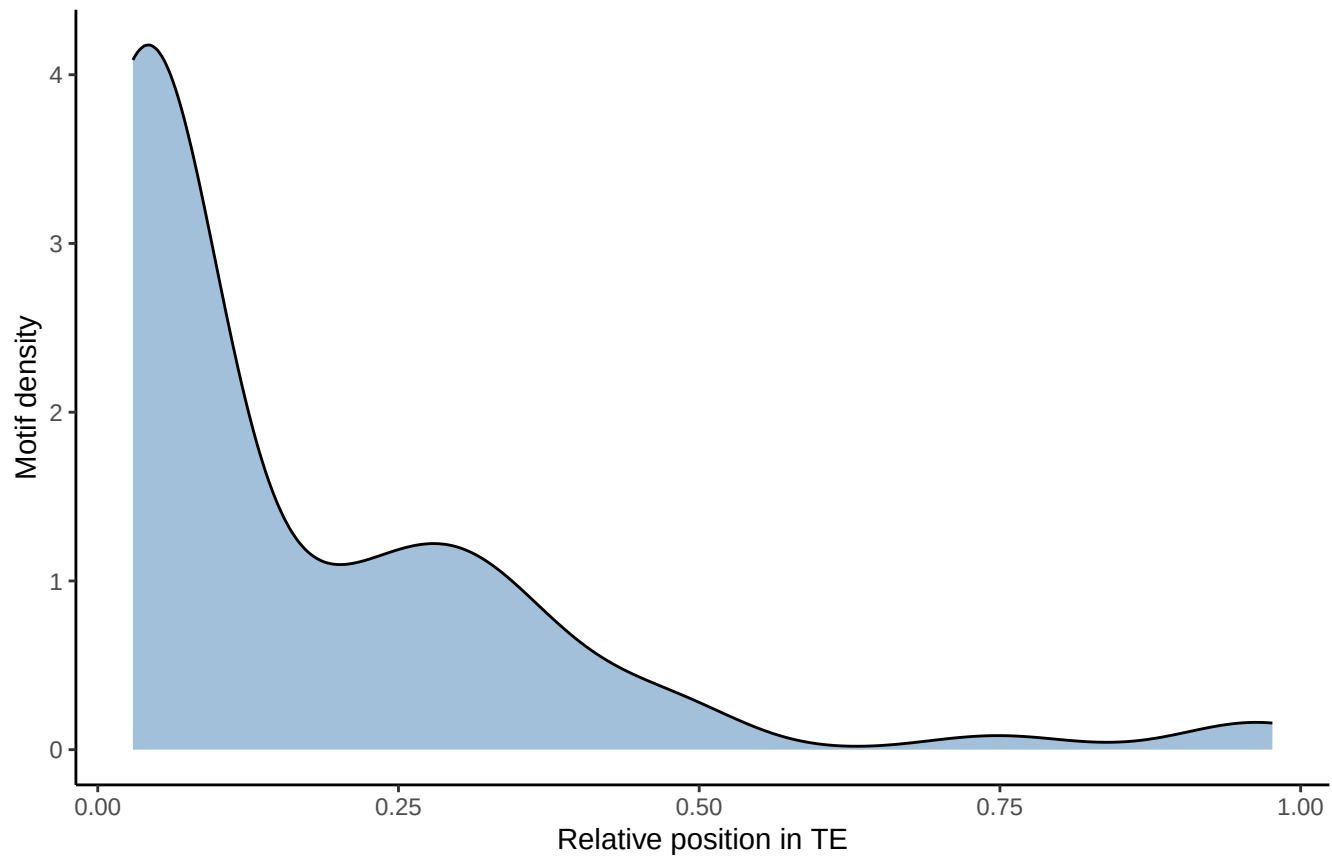
Motif distribution: fimo_out_35 MEME-31
