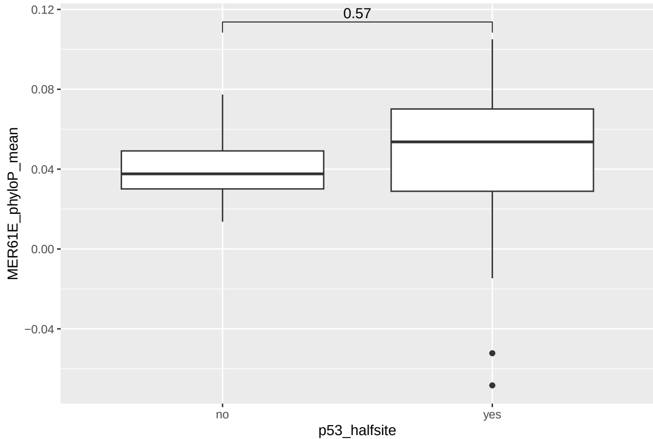
24T mean PhyloP score across my_MER elements with/without p53 halfsite
