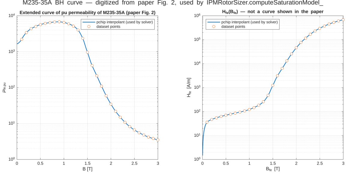
Figure 9: M235-35A BH curve digitized from the paper’s Fig. 2 (IPMRotorSizer.BFE_DATA/HFE_DATA), used internally by the saturation model. Left: \mu_{fe,pu} vs. B , same axes as the paper’s own figure. Right: H_{fe}(B) , the orientation the solver actually interpolates on.
