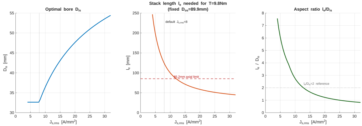
Figure 6: Sensitivity of the Formula 2 to the current density J_s . Raising it to \approx 12\text{A/mm}^2 brings l_e down to our 85.2\text{mm} target.
