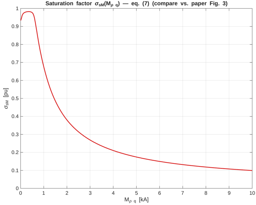
Figure 10: q-axis saturation factor \sigma_{sM}(M_q) (eq. 7), eye-comparable against the paper’s own Fig. 3.
