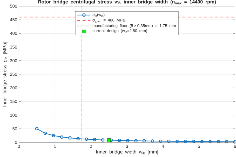
Figure 8: Inner bridge stress \sigma_{ib} vs. bridge width w_{ib} ( rotor_bridge_stress_sweep.m ) at this project’s own design point and n_{max} = 14,400 rpm, against the M235-35A yield line and the paper’s w_{ib} = 5w_{ob} manufacturing-floor rule. The margin to yield stays large across the whole swept range – the bridge is not the constraining factor for this design.
