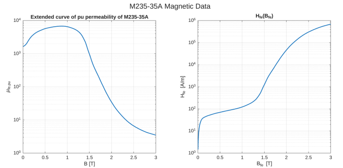
Fig. 8. M235-35A pu permeability and H_{fe}(B) curve, the latter used by the saturation model solver.
