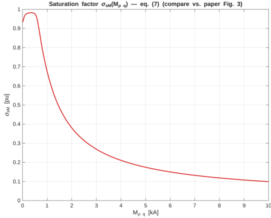
Fig. 10. q-axis saturation factor \sigma_{sM}(M_q) (eq. 7), eye-comparable against the paper's own Fig. 3.
