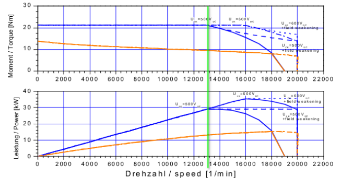
Fig. 4. From datasheet: Power and Torque vs Speed for the current motor. We focus on the U = 500 V_{DC} blue line. The green line marks the knee point where the motor enters field-weakening mode.
