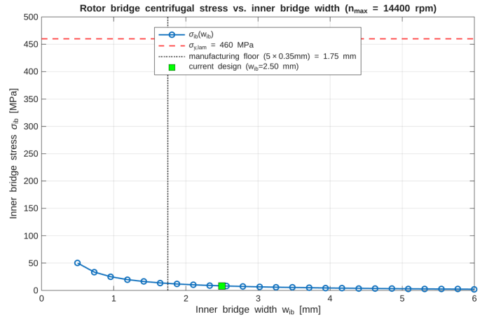
Fig. 9. Inner bridge stress \sigma_{ib} vs. bridge width w_{ib} ( rotor_bridge_stress_sweep.m ) at this project's own design point and n_{max} = 14,400 rpm, against the M235-35A yield line and the paper's w_{ib} = 5w_{ob} manufacturing-floor rule. The margin to yield stays large across the whole swept range; the bridge is not the constraining factor for this design.
