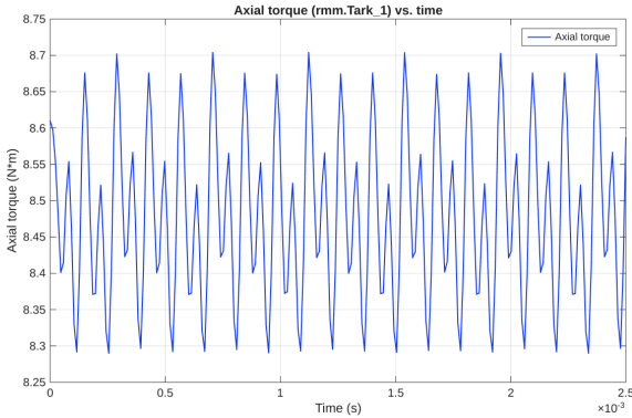
Fig. 11. Axial torque (rmm.Tark_1) over the time-dependent sweep.
