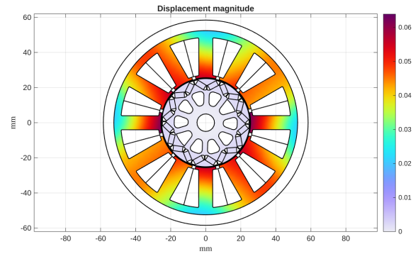
Fig. 14. Displacement magnitude from the coupled structural solve.
