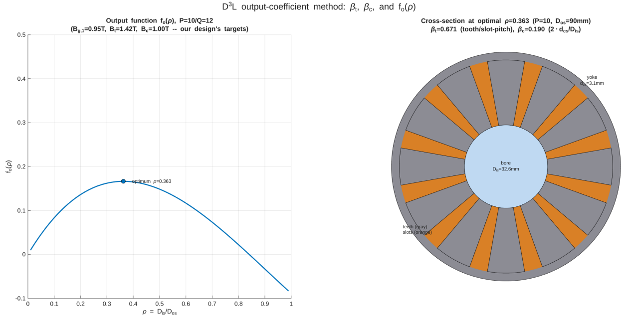
Fig. 5. Left: output function f_o(\rho) at our design's flux-density targets, dot marking the optimum. Right: cross-section schematic at that optimal ratio.
