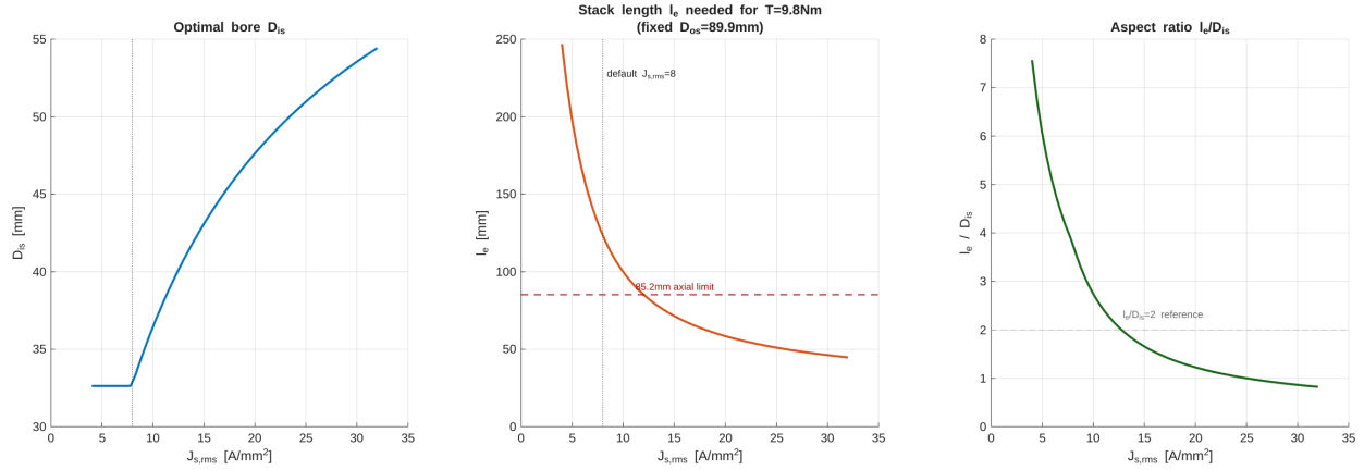
Fig. 6. Sensitivity of the Formula 2 to the current density J_s . Raising it to \approx 12\text{A/mm}^2 brings l_e down to our 85.2 mm target.
