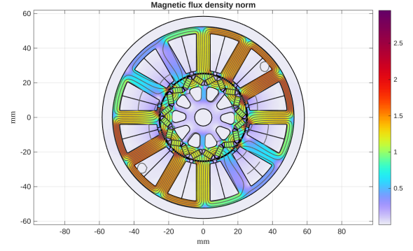
Fig. 12. Magnetic flux density norm with field lines, at the swept operating point.
