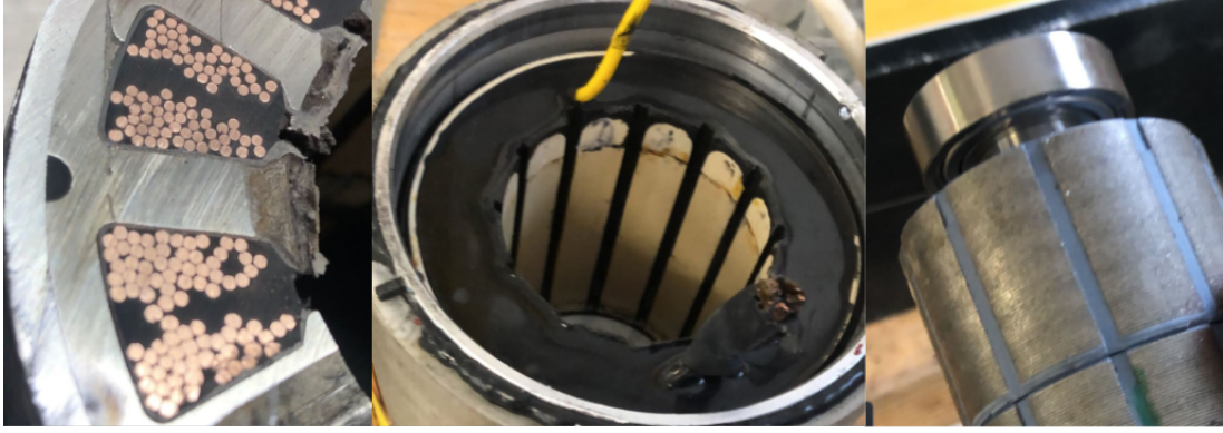
Fig. 1. Left: Traversal cut of the stator. Center: Stator. Right: Rotor.
