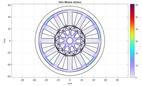
Fig. 13. Von Mises stress distribution from the coupled structural solve.
