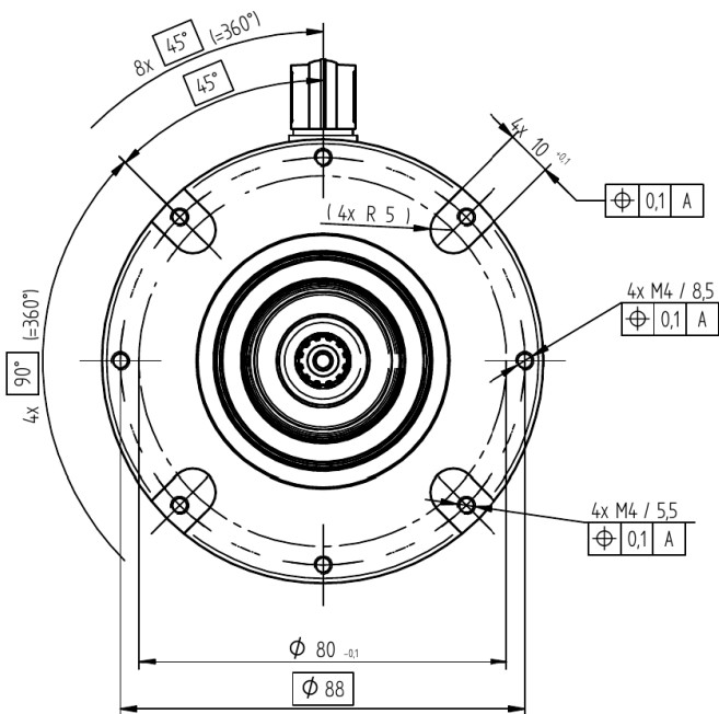
Fig. 3. Front view of the current motor.
