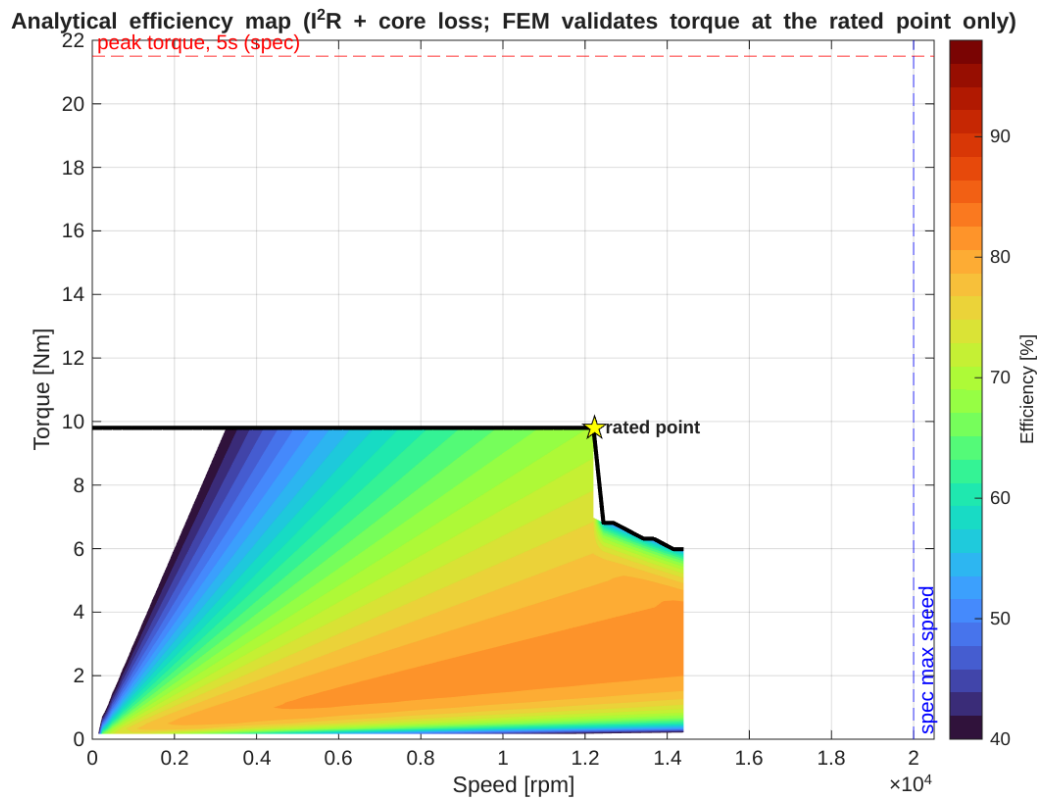
Fig. 15. Analytical efficiency map over the torque-speed envelope (EfficiencyMapSizer.plotMap). Black line: achievable envelope. Star: rated design point.
