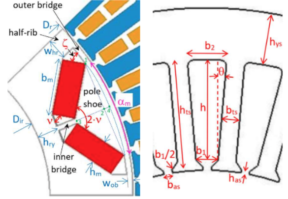
Fig. 7. V-Shape IPM Motor Layout
