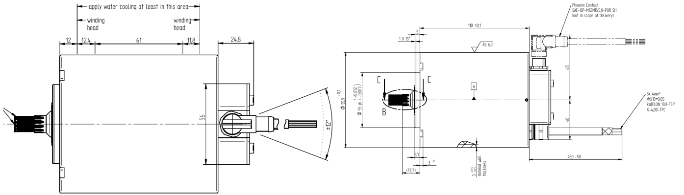
Fig. 2. Side view of the current motor.
