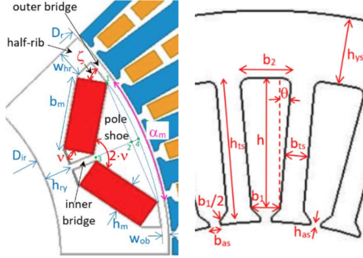
Figure 7: V-Shape IPM Motor Layout
