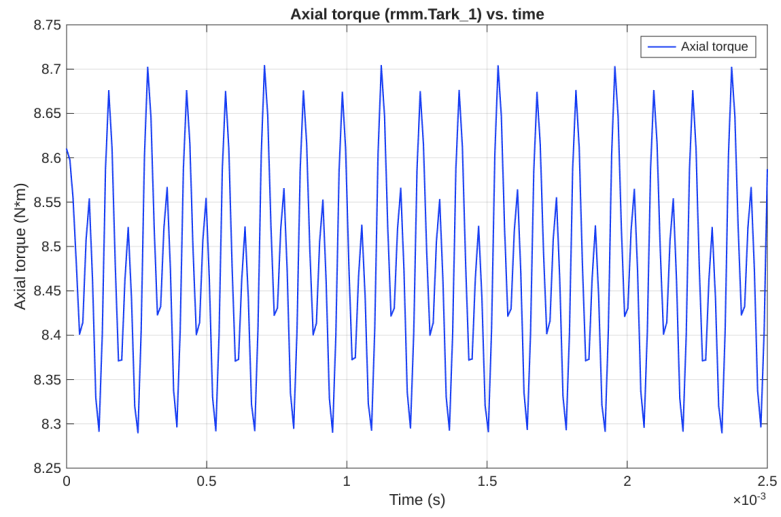
Figure 11: Axial torque ( rmm.Tark_1 ) over the time-dependent sweep.
