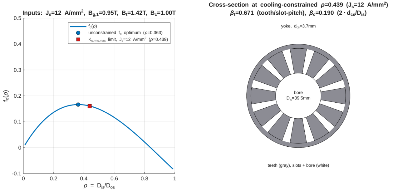
Fig. 6. Left: Optimum dimeter ratio optimum. Right: cross-section actual dimensions at optimal ratio.
