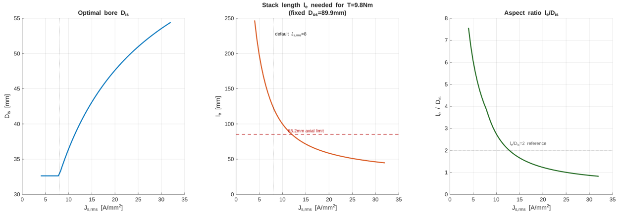
Fig. 5. Sensitivity of the Formula 2 to the current density J_s . Raising it to \approx 12 \text{ A/mm}^2 brings l_e down to our 85.2 mm target.
