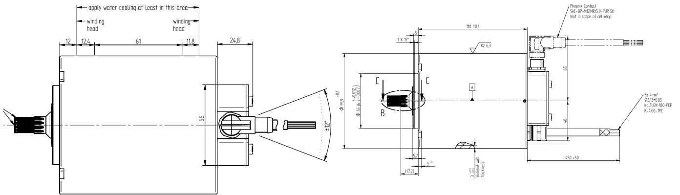
Fig. 2. Side view of the current motor.
