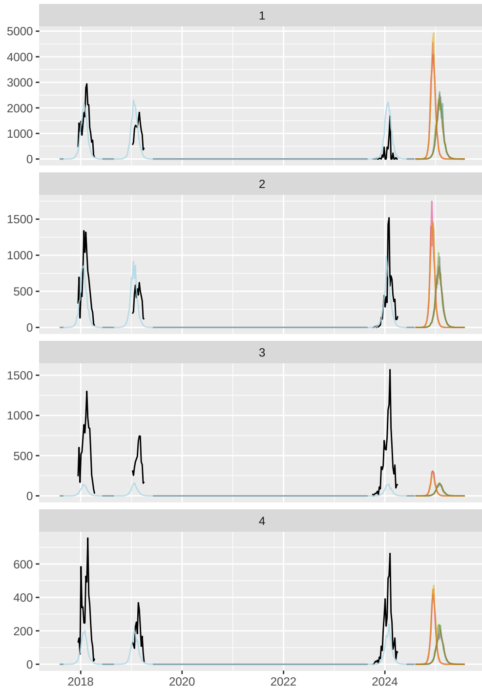
Austria (AT), ILI rate
