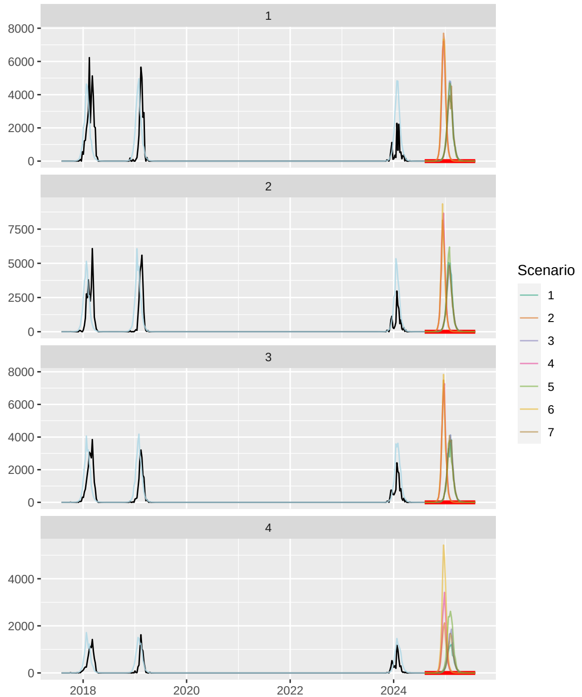
Belgium (BE), ILI incidence
