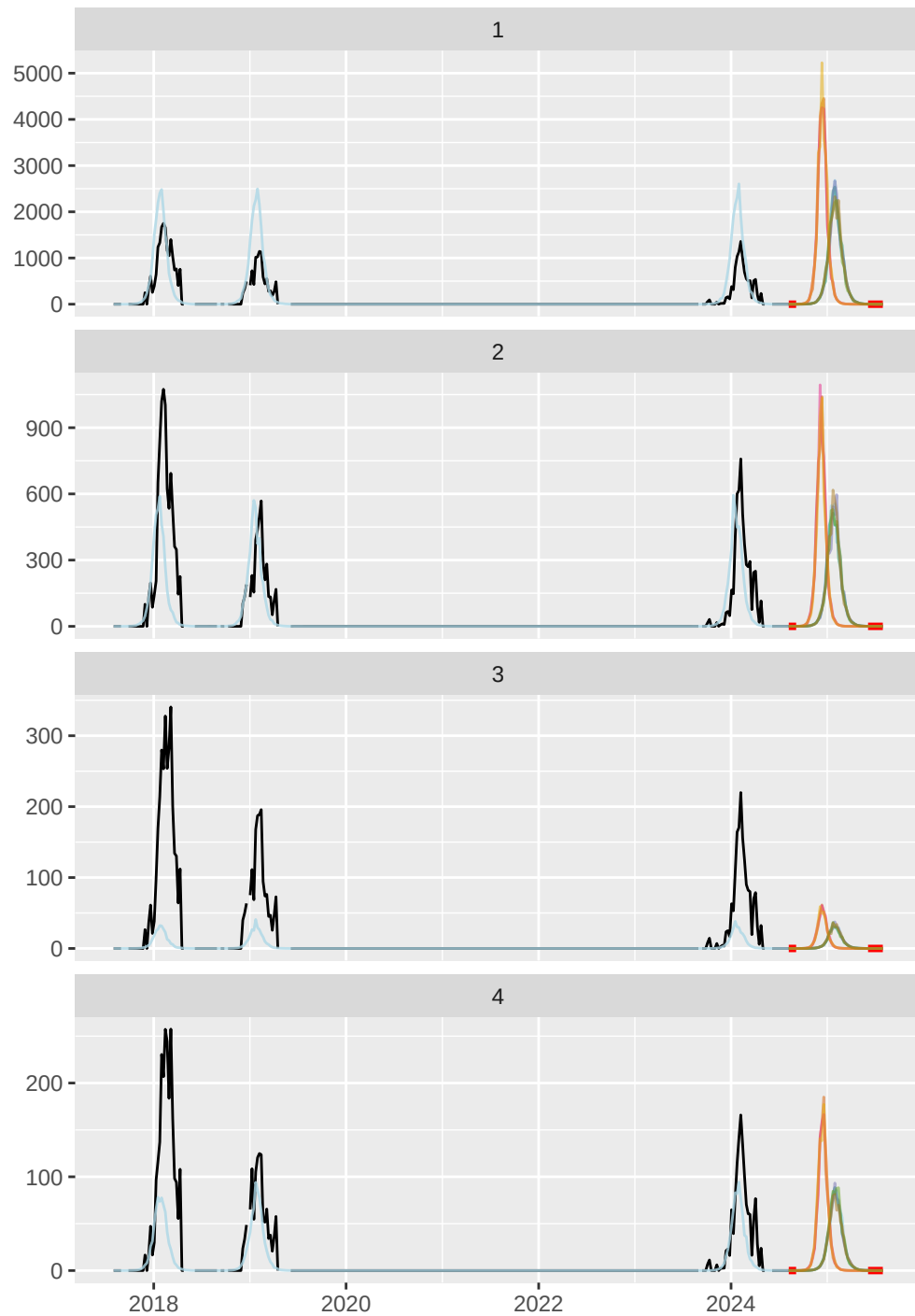
Poland (PL), ILI rate
