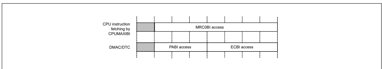
Figure 15.3 Example of parallel operations
