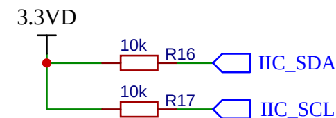
IIC上拉电阻
