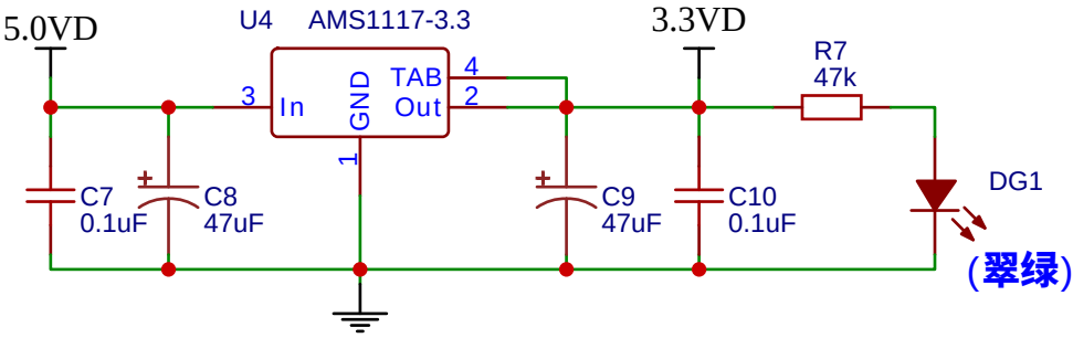
电源3.3V
