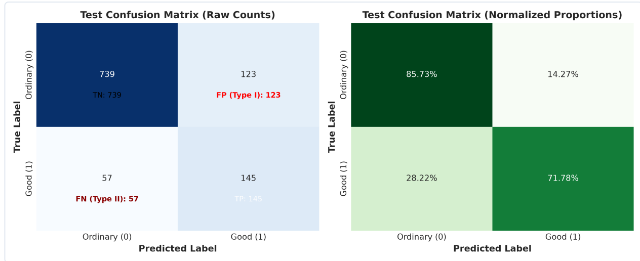
figure_02_confusion_matrix.png
