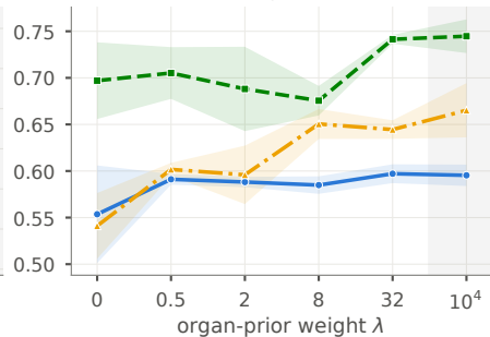
Merlin / SegVol, B = 256
