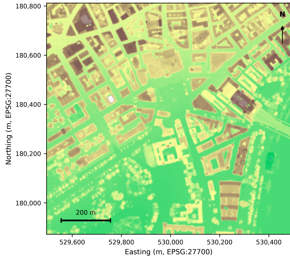
(a) North-up DSM
