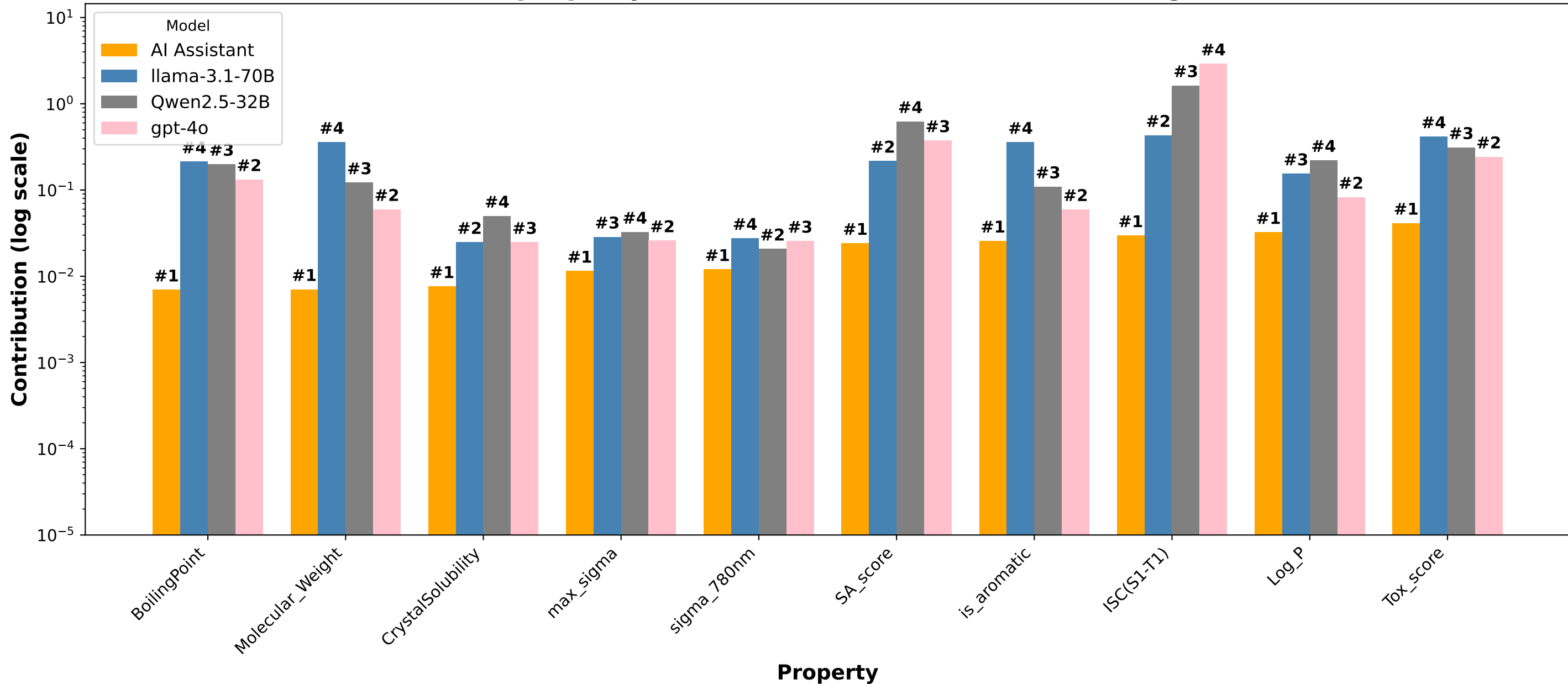
Per-property contribution to wMAE with Rankings
