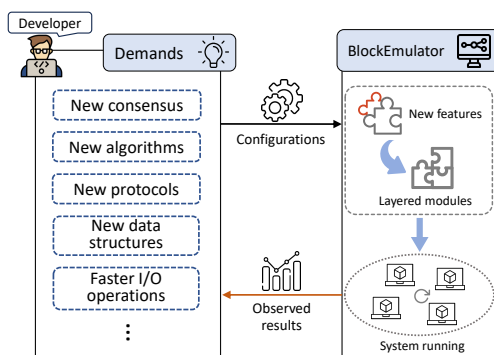
图 1.1: The design principle of BlockEmulator.
