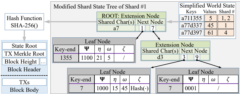
图 2.3: Data structure of the modified Shard State Tree (mSST).
